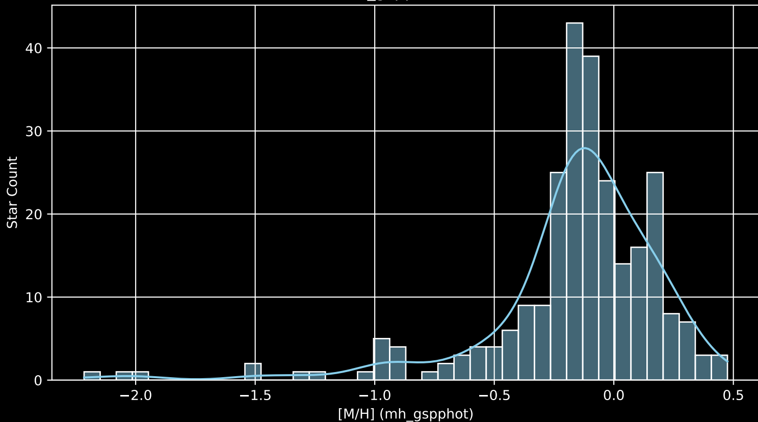
APOGEE DR17 Field: [Berkeley_22_btx [M/H] (mh_gspphot) (n= 262)
