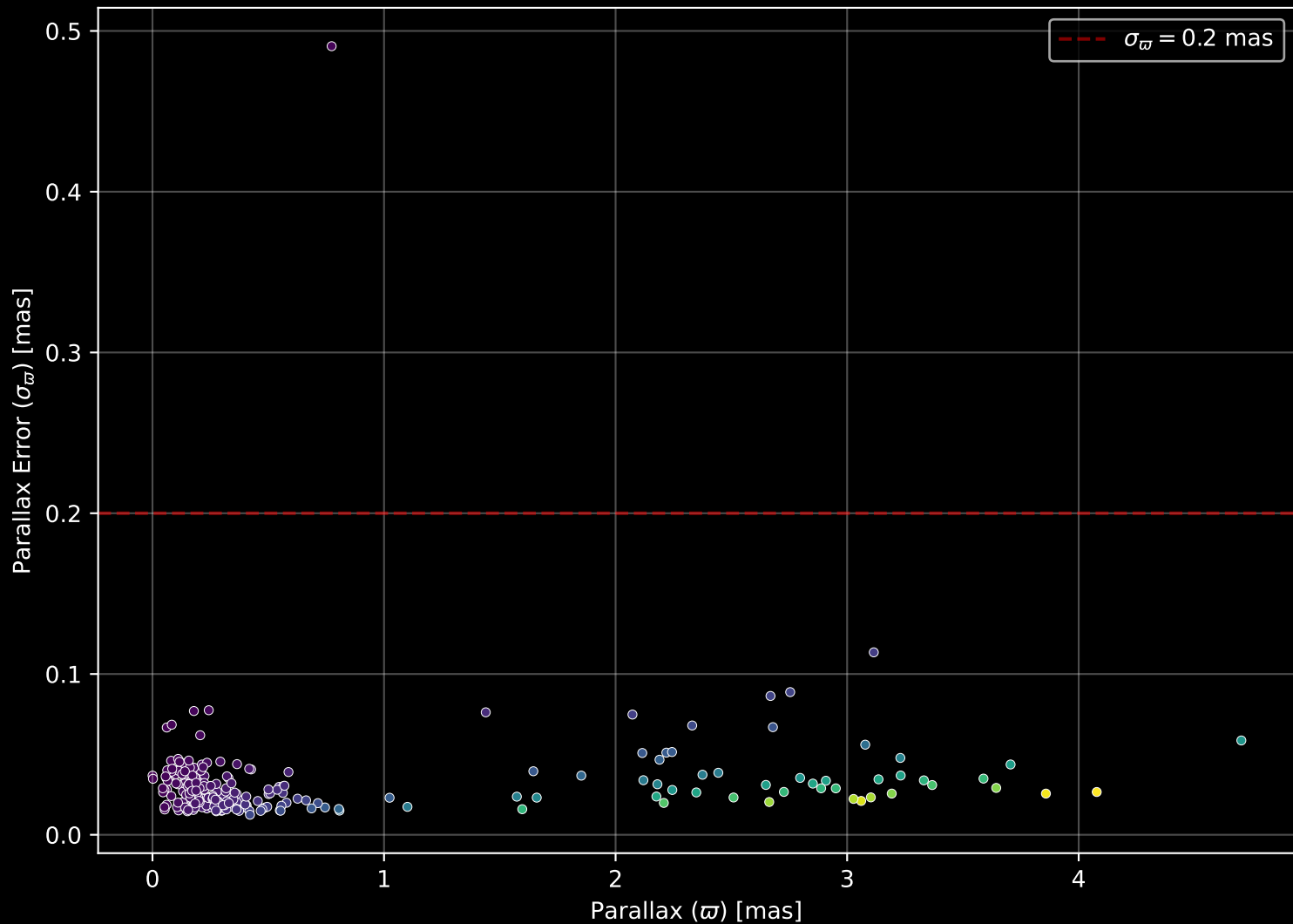
APOGEE DR17 Field: [Berkeley_22_btx] Parallax Quality (n= 263)
