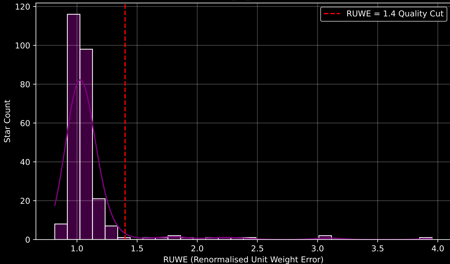
GAPOGEE DR17 Field [Berkeley_22_btx] RUWE Distribution (n= 263)
