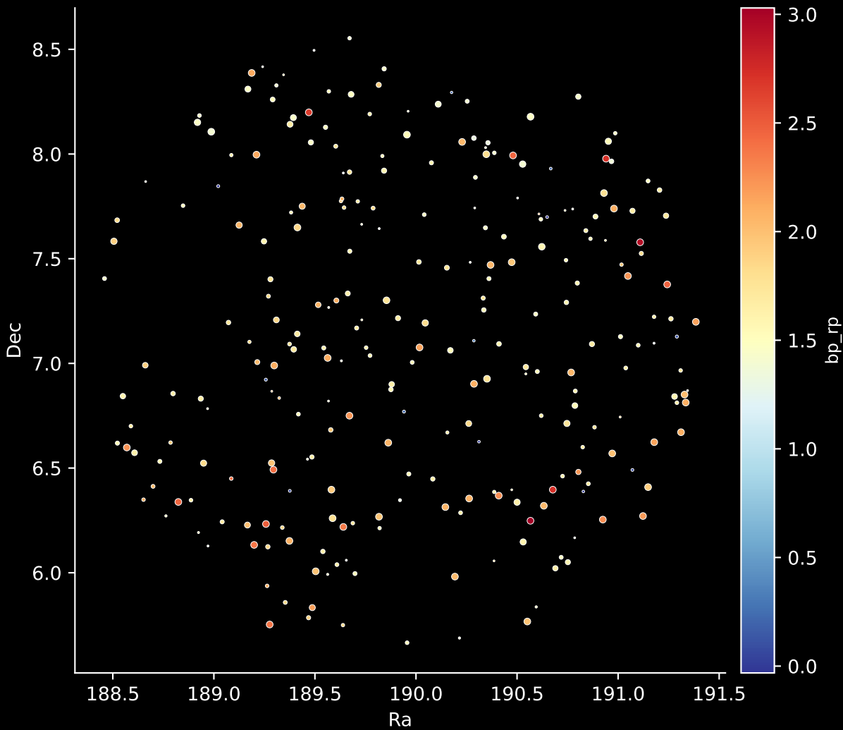
APOGEE DR17 Field: [Berkeley_22_btx] Stars: 263
