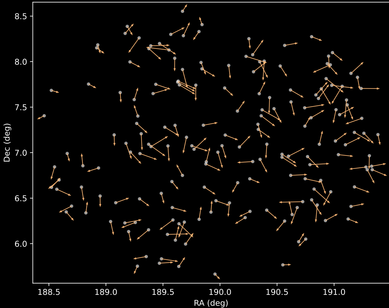
APOGEE DR17 Cluster 3 Proper Motion Vectors (n=177)
