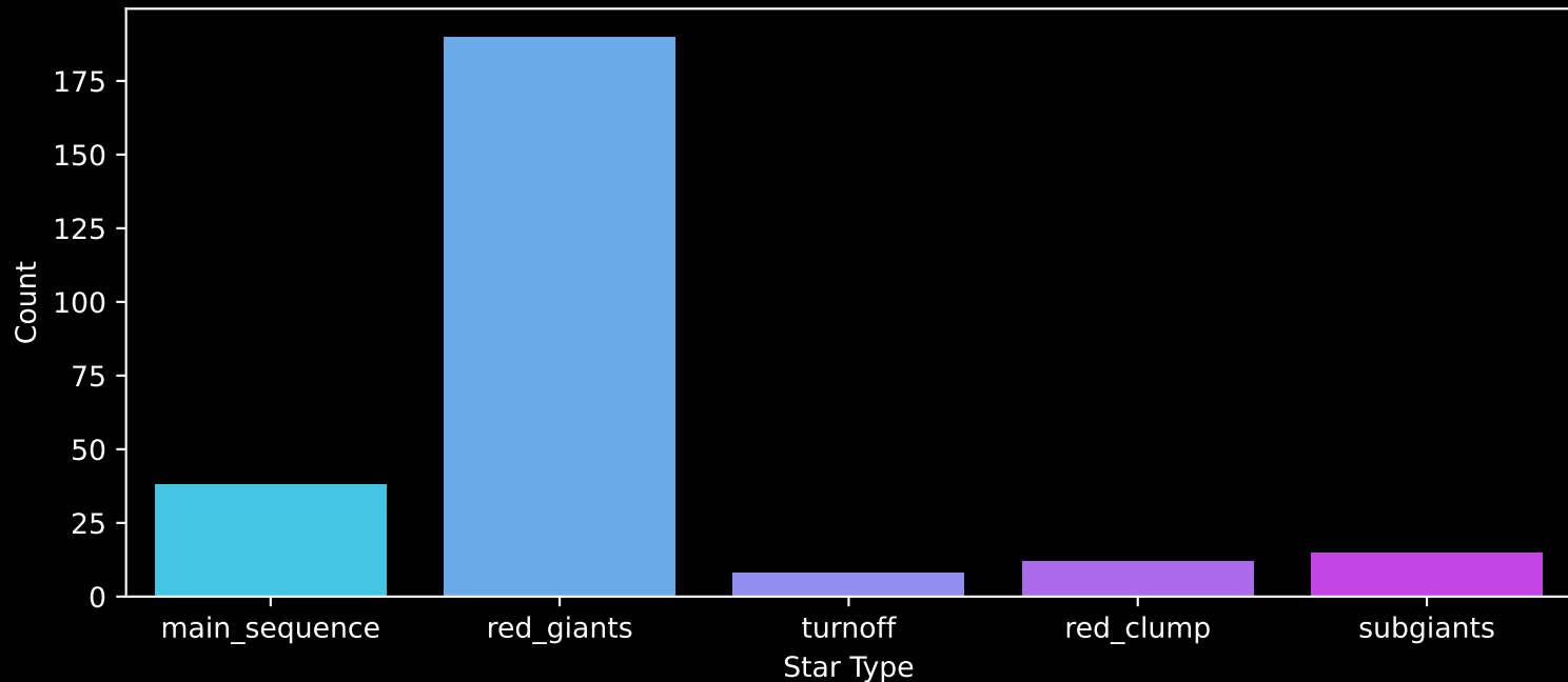
APOGEE DR17 Field: [Berkeley_22_btx] Count plot of Star Type
