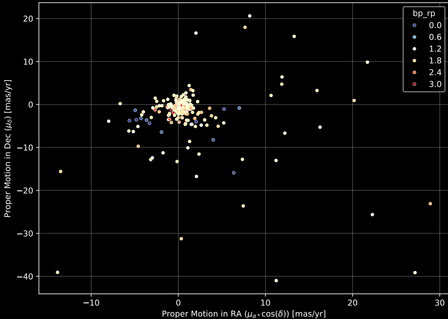
APOGEE DR17 Field: [Berkeley_22_btx] Proper Motion Diagram (n= 263)
